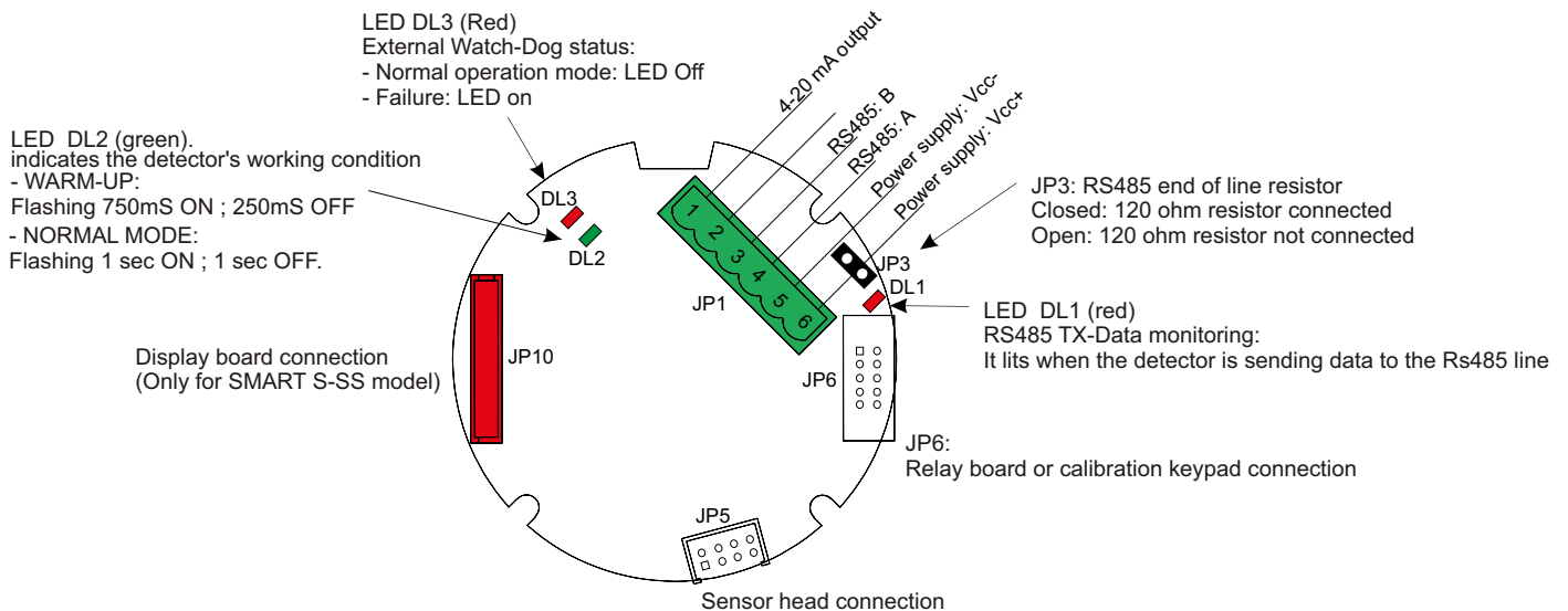
Figure 1) Detector circuit layout without HART module
